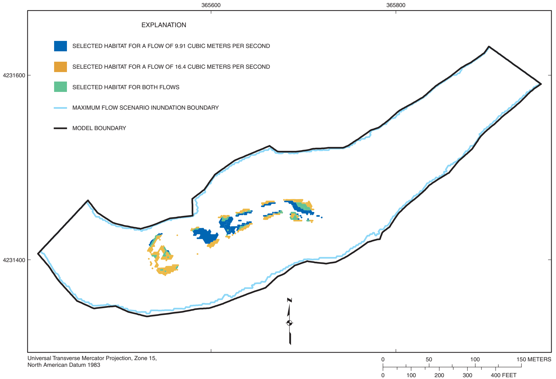
Figure 4-61. Selected habitat area distribution for habitat categories 16, 17 combined (channel catfish) at flows of 9.91 and 16.4 cubic meters per second at Marais des Cygnes River site MDC2.
